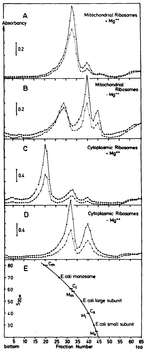
Fig. 1. Sucrose density gradient centrifugation of mitochondrial and cytoplasmic ribosomes. ●—●: absorbance at 260 nm; ○---○: absorbance at 280 nm.
